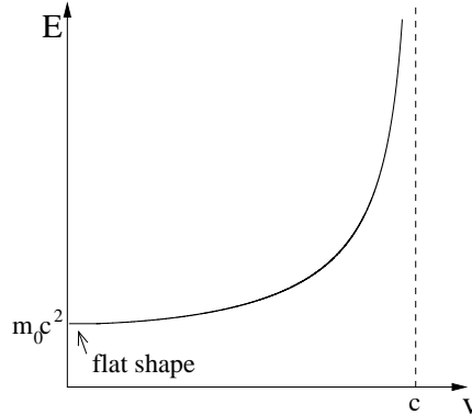
Figure 4: E vs v for a massive particle
