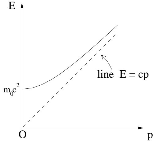
Figure 1: E vs p for a massive particle
