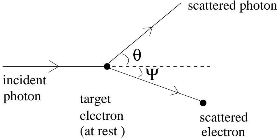
Figure 5: The schematics of Compton scattering
