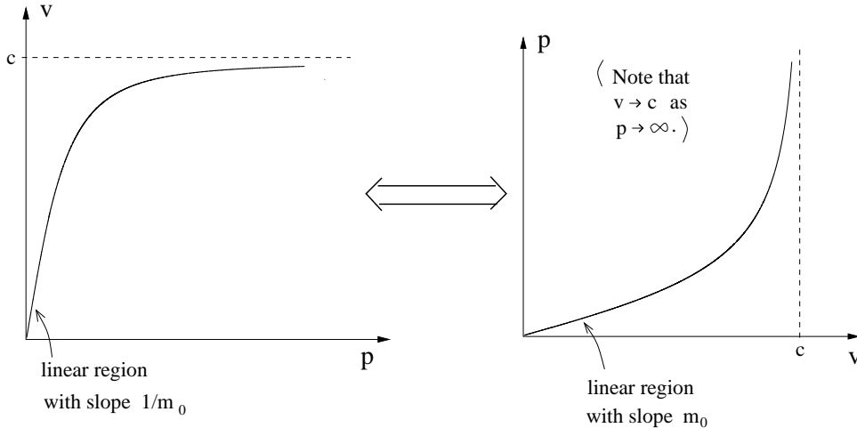
Figure 3: v vs p and p vs v for a massive particle
