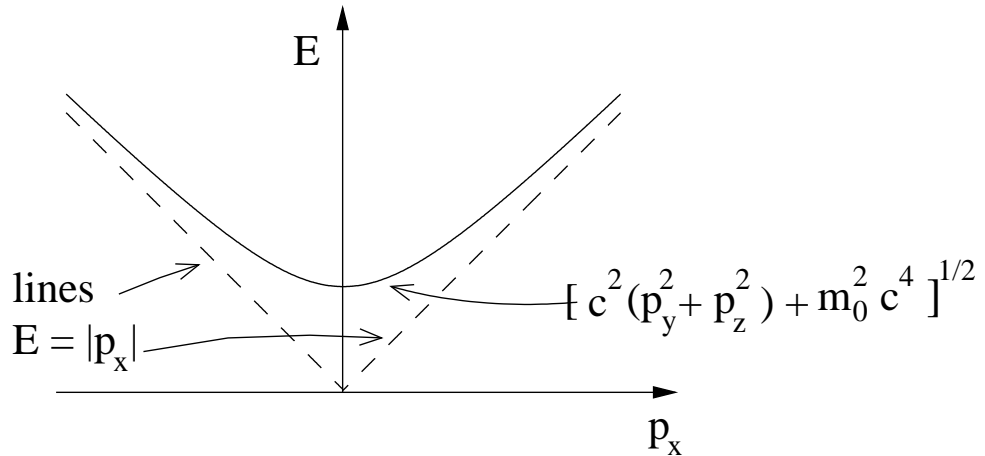
Figure 2: E vs p_x (with fixed p_y and p_z ) for a massive particle
