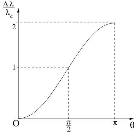
Figure 6: \frac{\Delta\lambda}{\lambda_c} vs \theta
